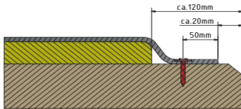
Cross section in mm specification
